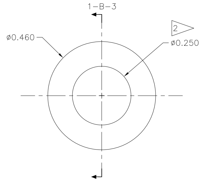
END VIEW 1-B-5 FELT WIPER SEAL
